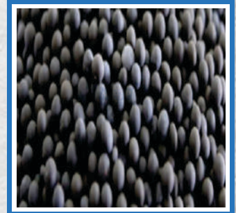
PALLADIUM CATALYST
